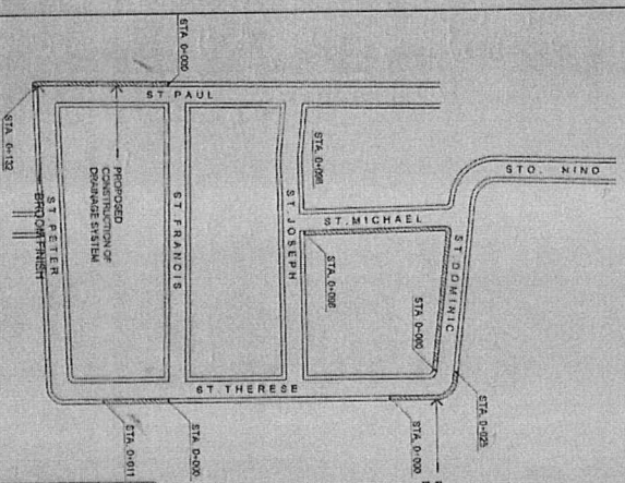
PLAN SCALE 1:12.5
